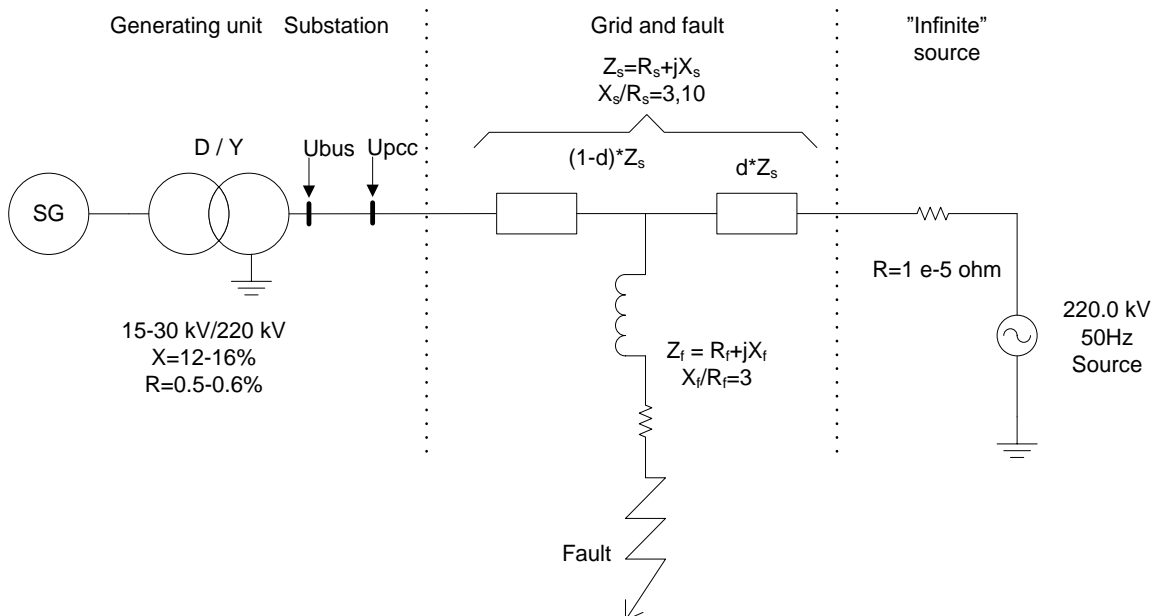
(b) Synchronous generator model acceptance set-up
