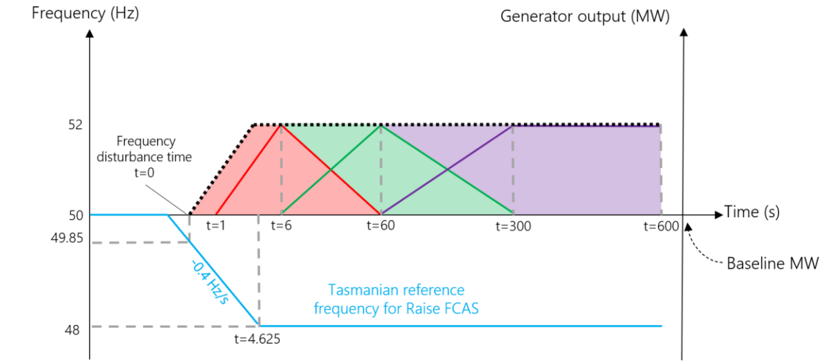
Figure 8 shows a visual representation of the measurements applied to verify that at least the minimum required Contingency FCAS has been delivered in each timeframe by an FCAS Provider also registered in the Very Fast FCAS markets.
