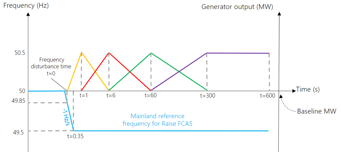
Figure 8 Measurement timeframes for Raise Contingency FCAS for the Mainland and Tasmania
