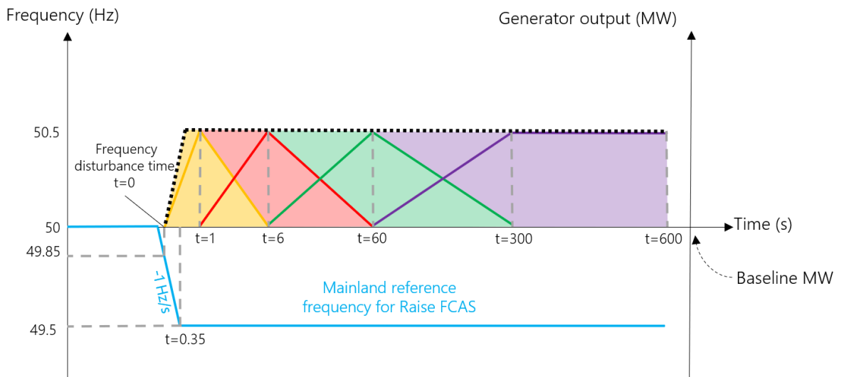
Figure 9 Combined measurement timeframes for Raise Contingency FCAS for Mainland and Tasmania
