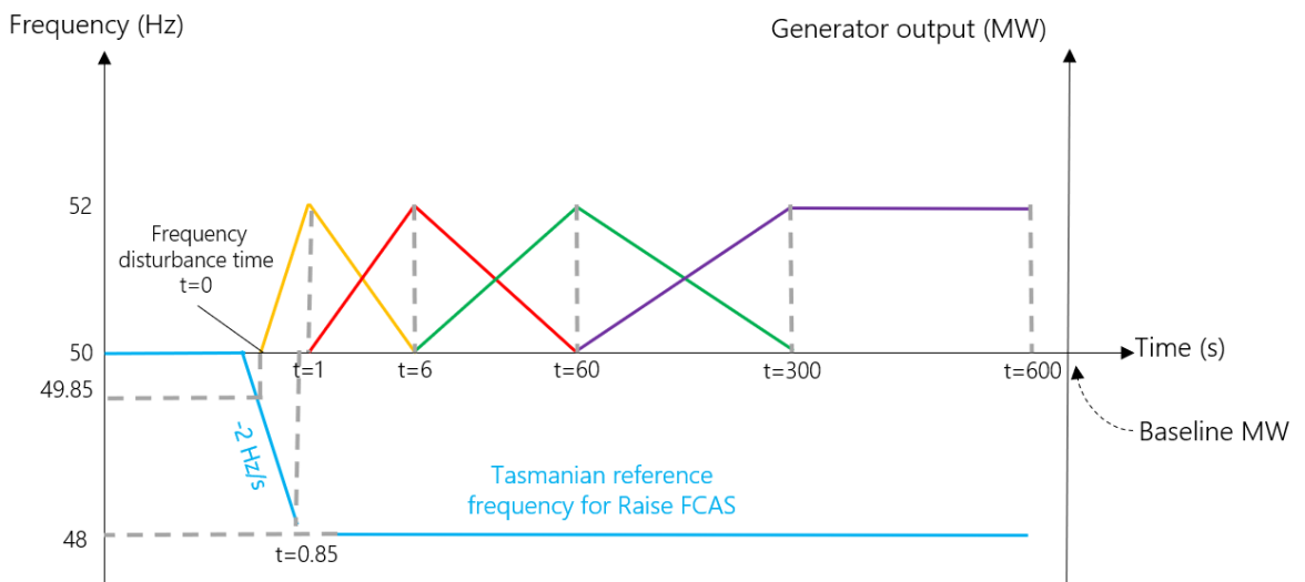
Figure 9 shows an example of how a simple Variable Controller that supplies a droop-based response to a Frequency Disturbance can deliver across the Contingency FCAS timeframes by an FCAS Provider also registered in the Very Fast FCAS markets.
