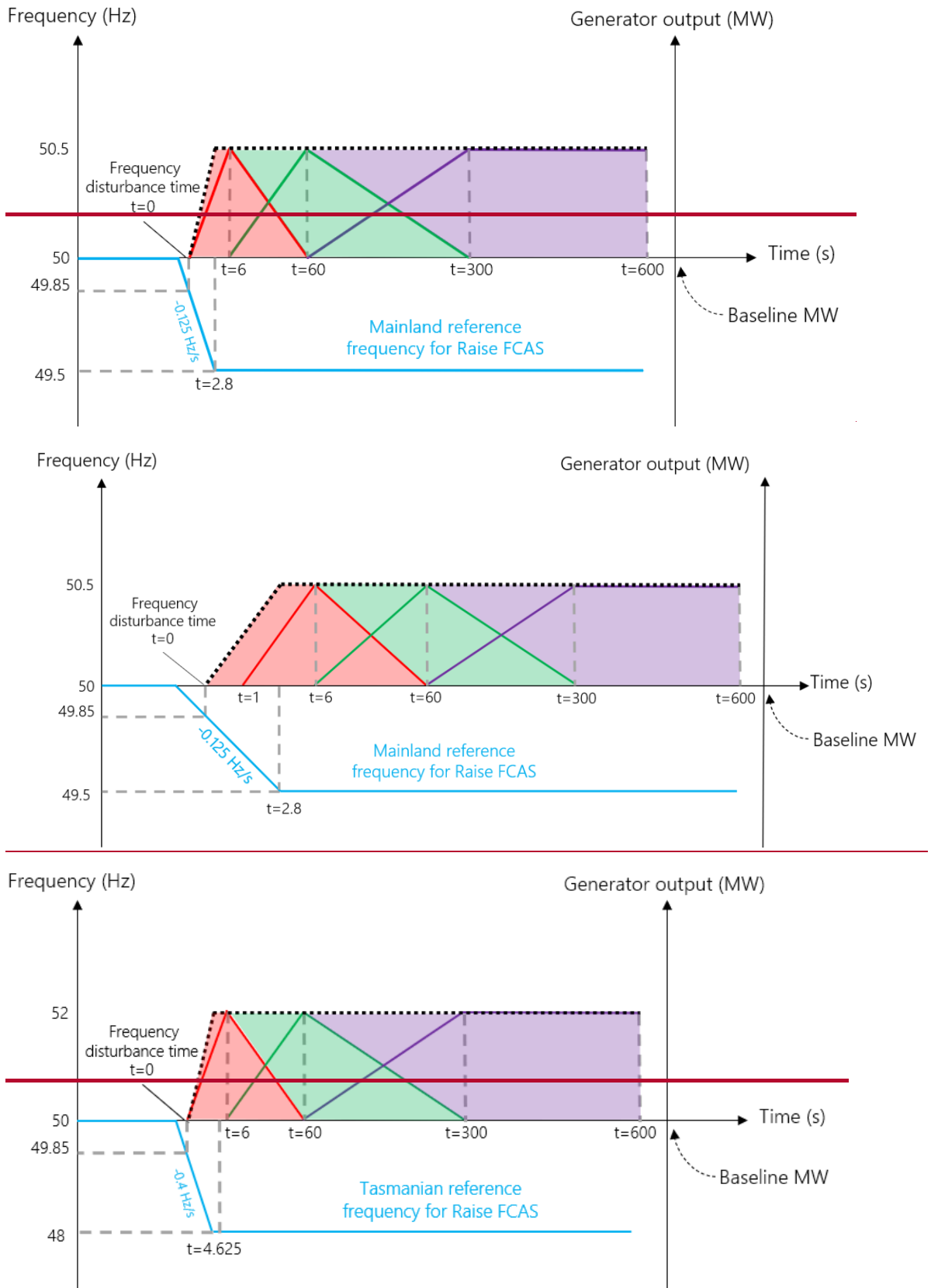
Figure 7 Combined measurement timeframes for Raise Contingency FCAS for Mainland and Tasmania
