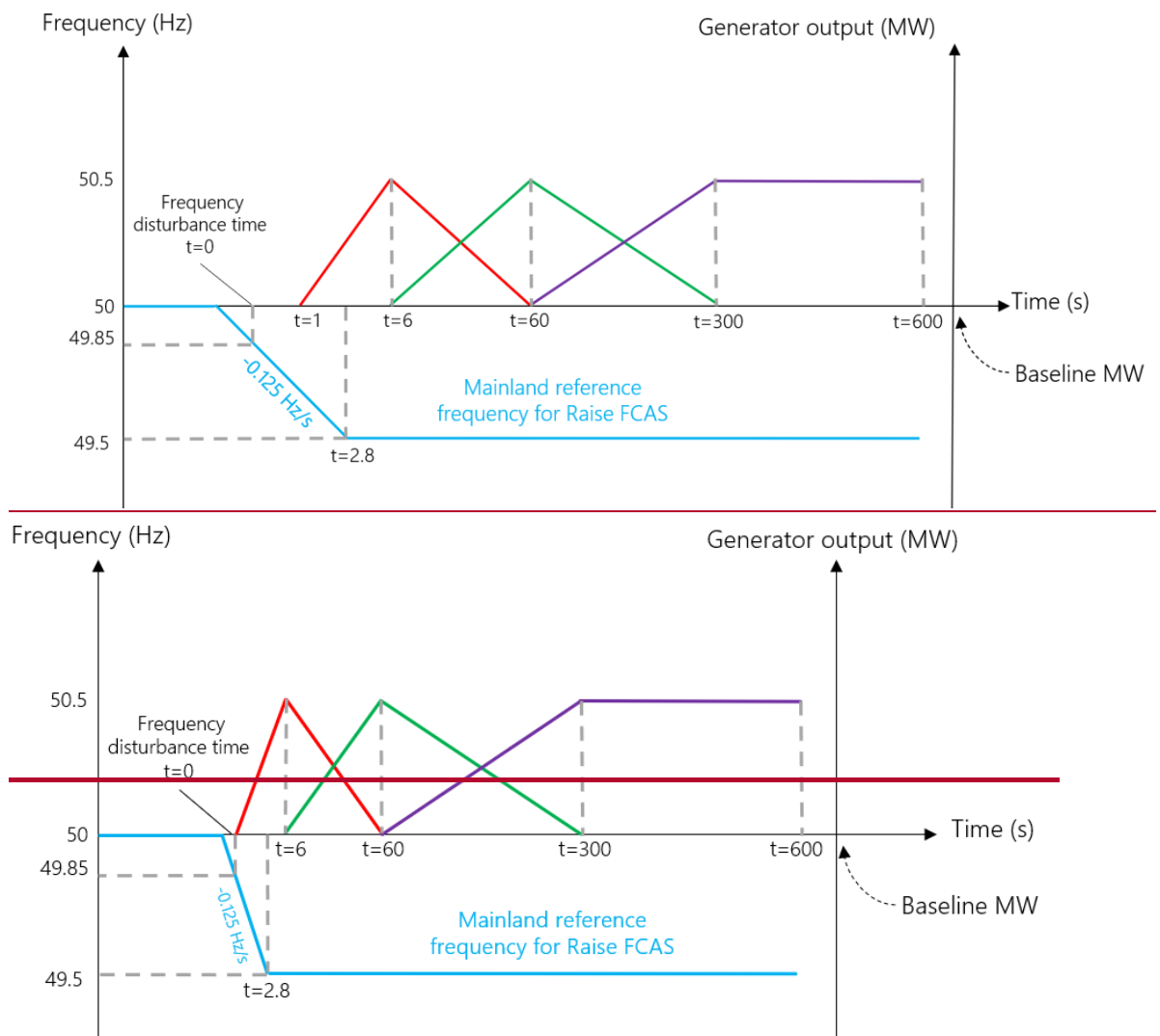
Figure 6 Measurement timeframes for Raise Contingency FCAS for the Mainland and Tasmania
