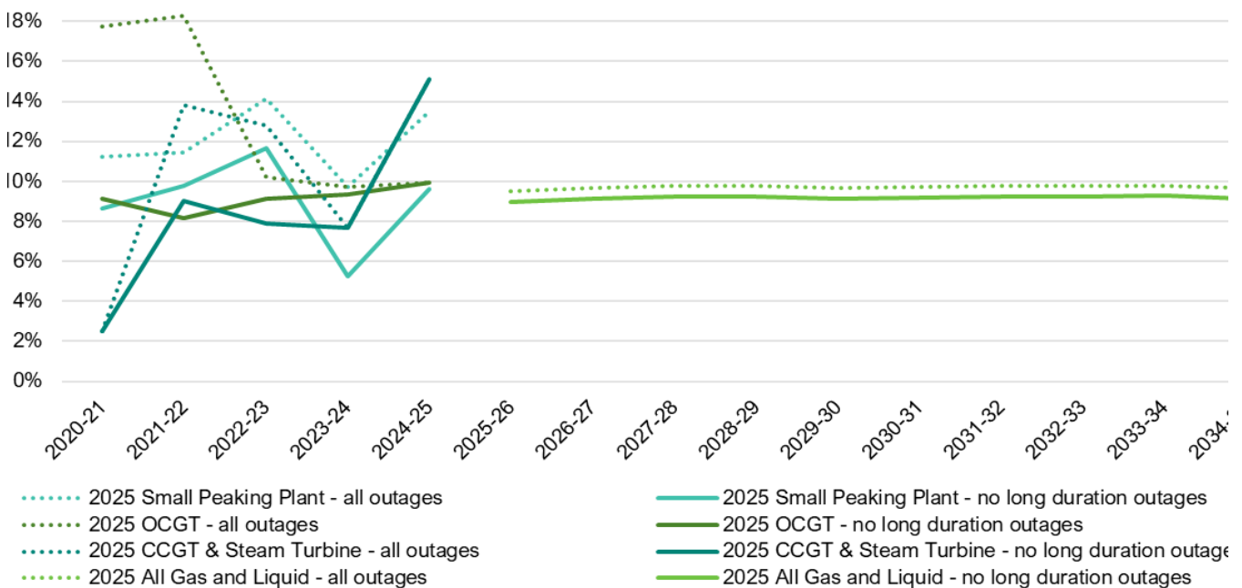
Figure 54 Equivalent full unplanned outage rate projections for open-cycle gas turbine, closed-cycle gas turbine and steam turbine generation and small peaking plant technologies
