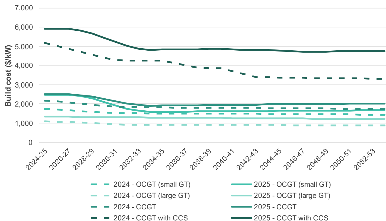
Figure 59 2024 versus 2025 Global NZE post 2050: build cost trajectories forecasts for gas generation
