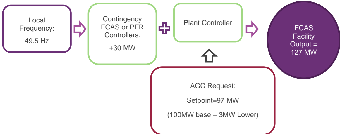
Figure 11 Co-ordinated output for FCAS Facility at 100 MW given Lower Regulation FCAS request of 3 MW while responding with 30 MW to a Frequency Disturbance
