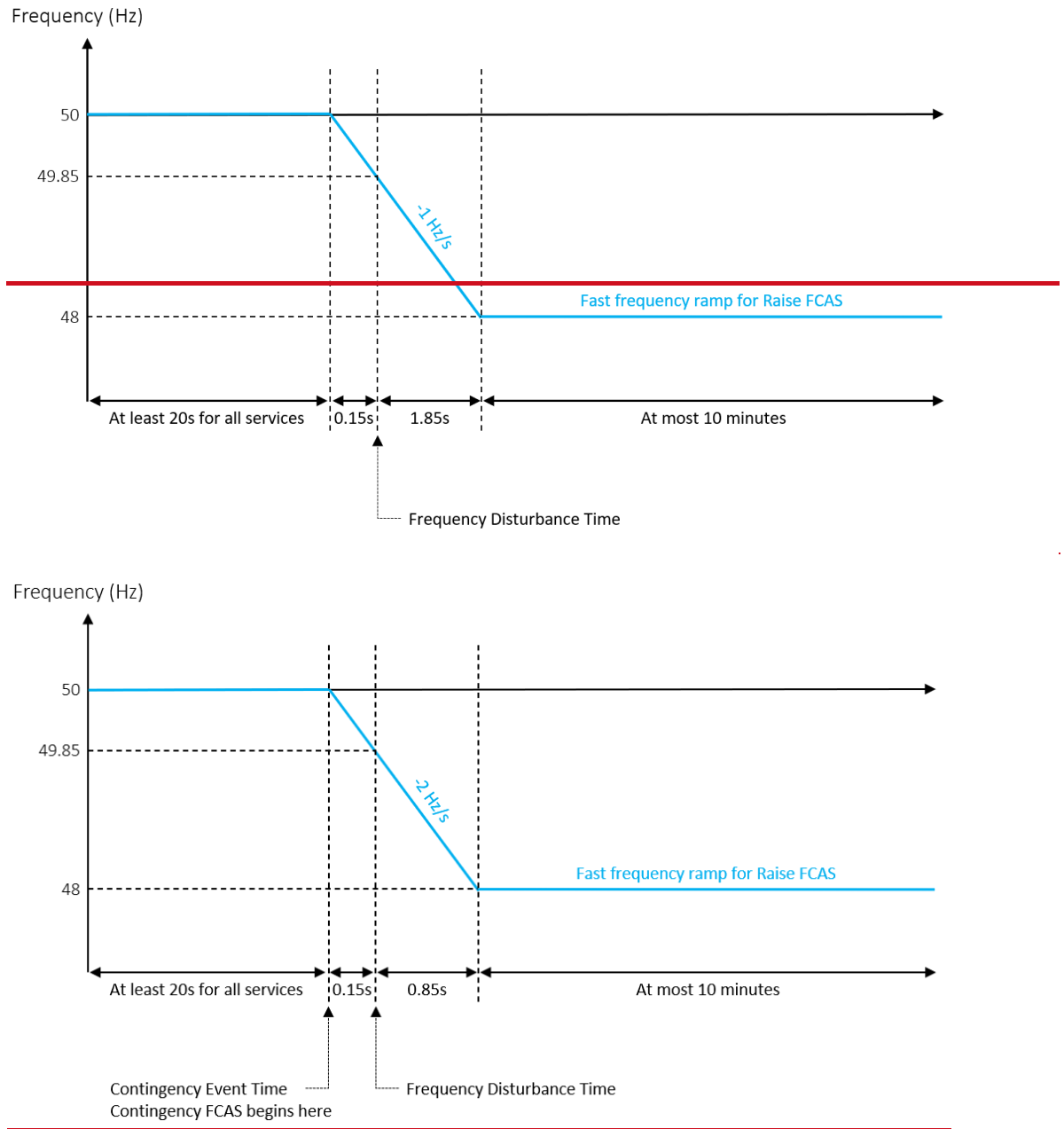
Figure 5 Fast Frequency Ramp for Tasmania
