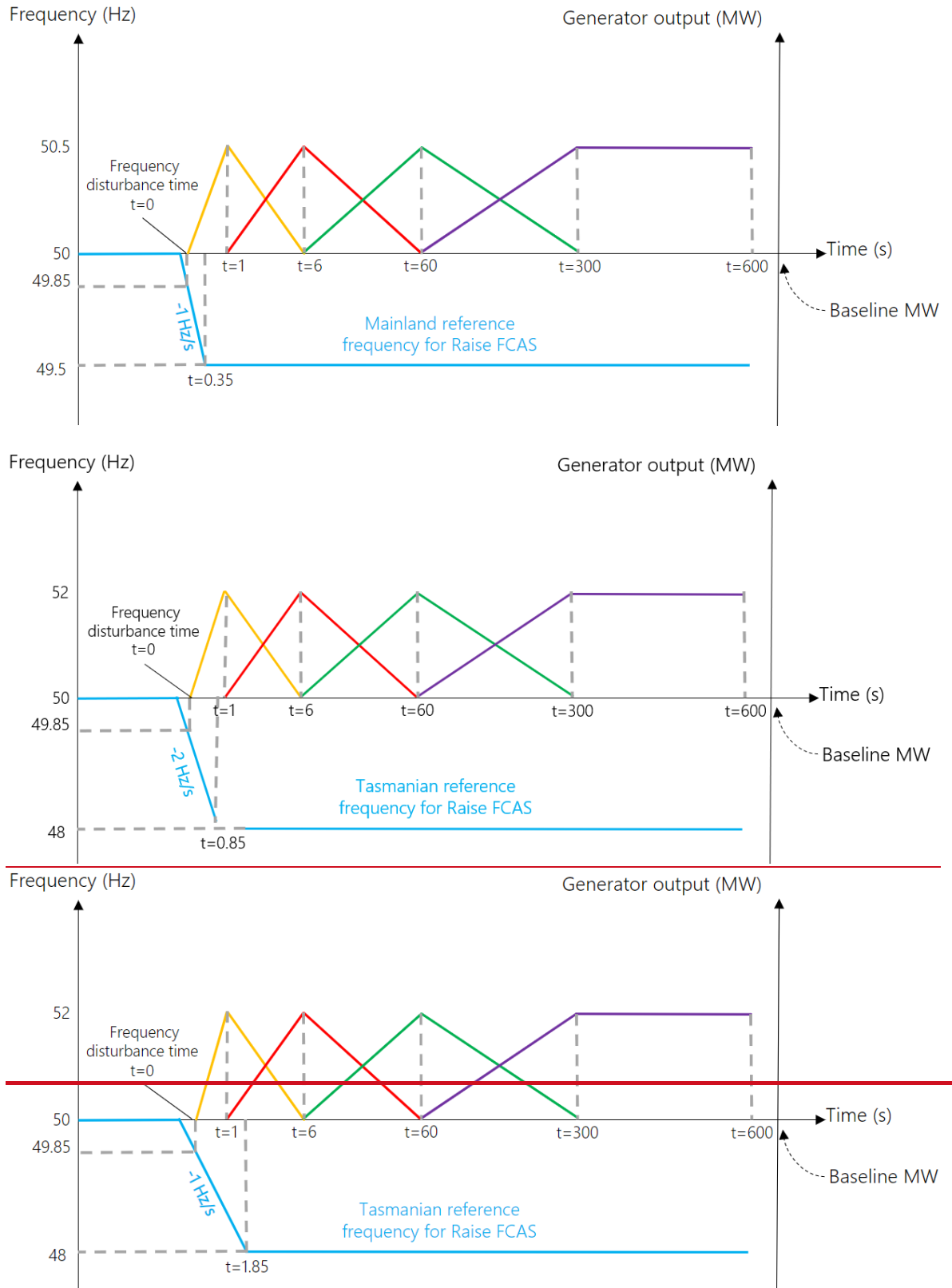
Figure 8 Measurement timeframes for Raise Contingency FCAS for the Mainland and Tasmania
