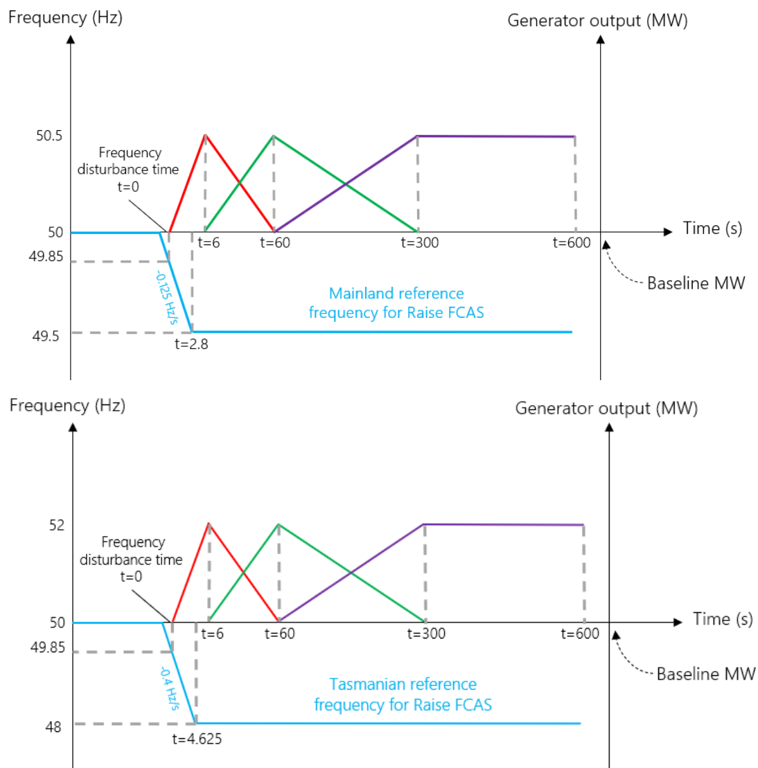
Figure 6 Measurement timeframes for Raise Contingency FCAS for the Mainland and Tasmania
