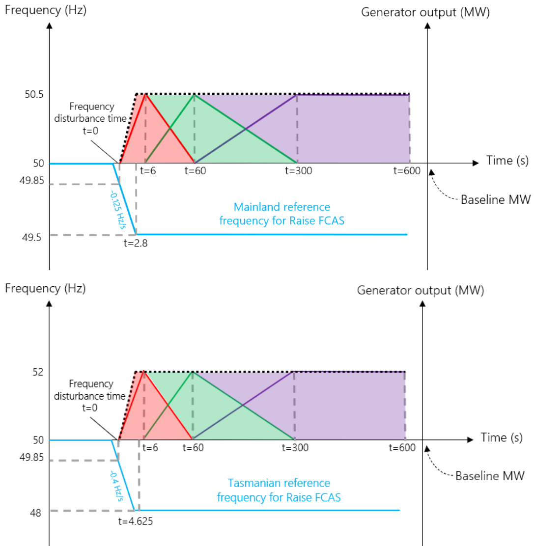
Figure 7 Combined measurement timeframes for Raise Contingency FCAS for Mainland and Tasmania
