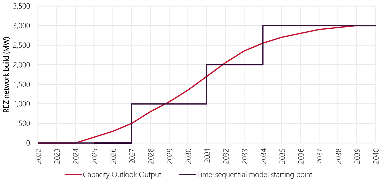
Figure 13 Figure 14 Conversion of linearised REZ expansion to network upgrade options
