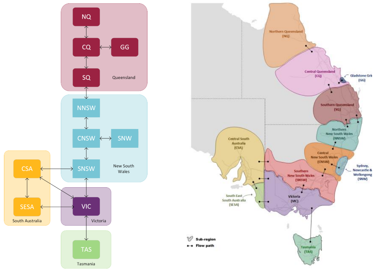
Figure 5 NEM sub-regional topology
