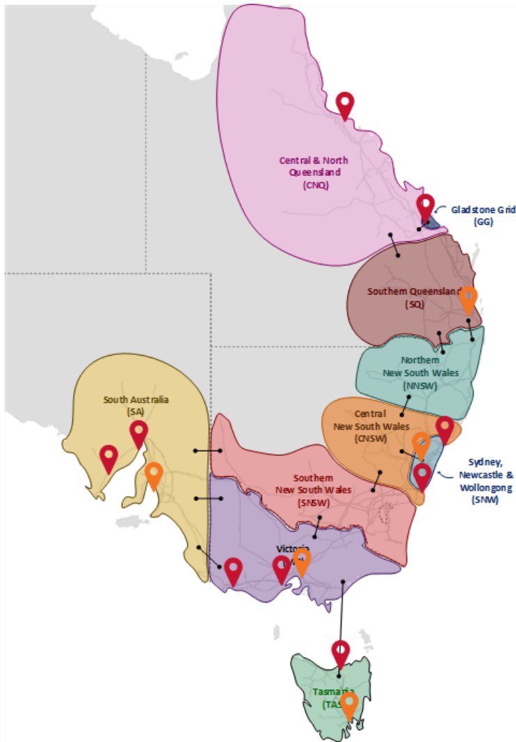
Figure 15 Figure 16 Electrolyser locations and their connections to electricity nodes
