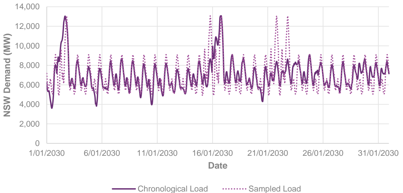
Figure 9 Figure 10 Example representation of a sampled load profile
