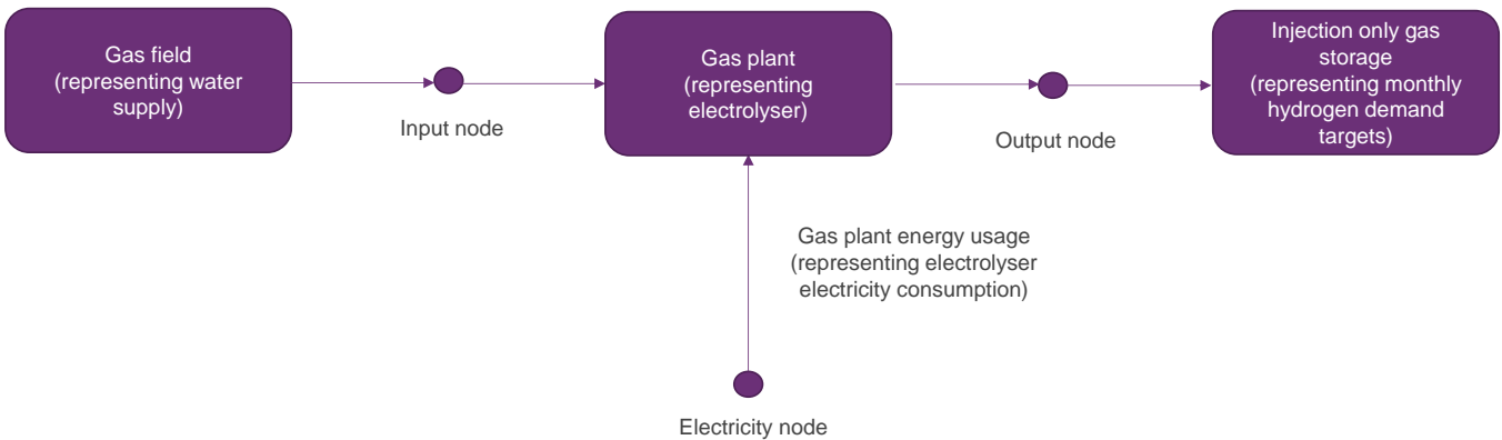
Figure 14 Figure 15 Hydrogen implementation in capacity outlook models
