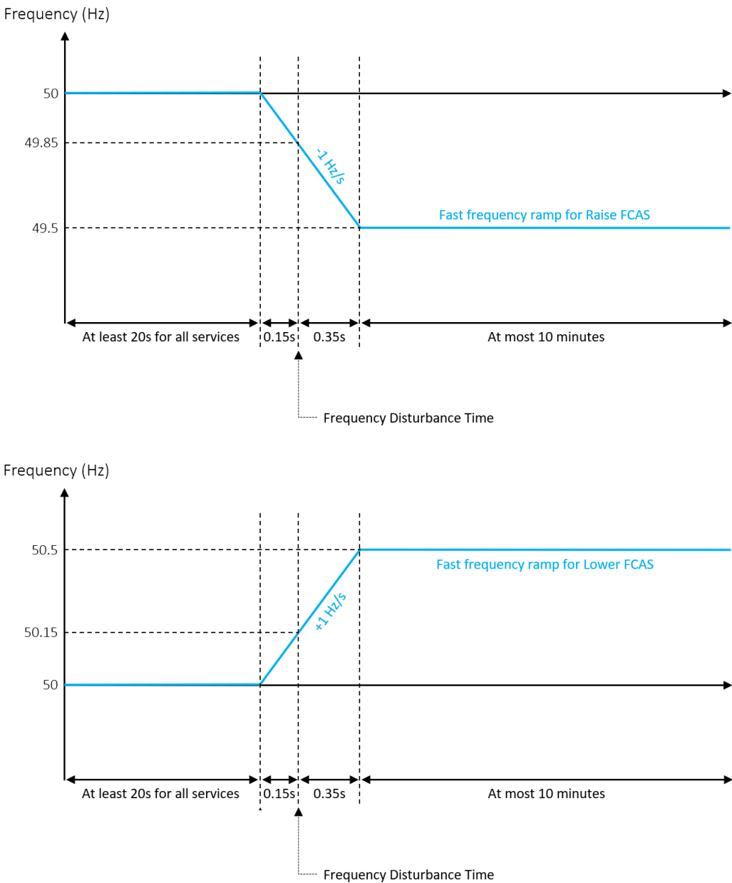
Figure 4 Fast Frequency Ramp for the Mainland
