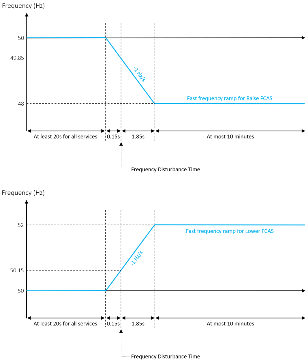
Figure 5 Fast Frequency Ramp for Tasmania
