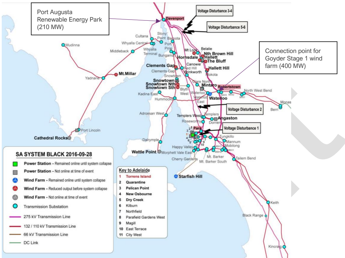
Figure 6 Map of South Australian transmission system showing location of 2016 black system event faults and significant new connections since 2019
