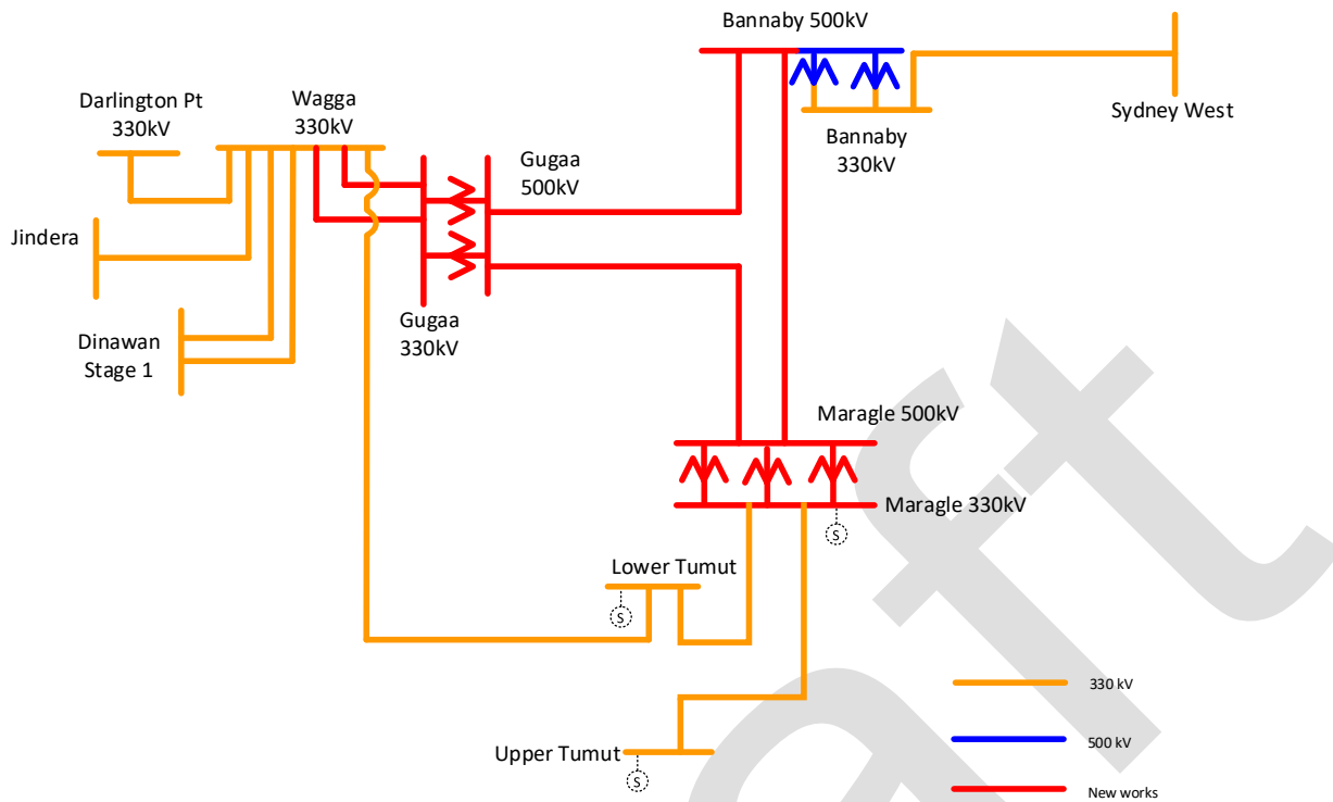
Figure 4 HumeLink augmentation simplified single line diagram
