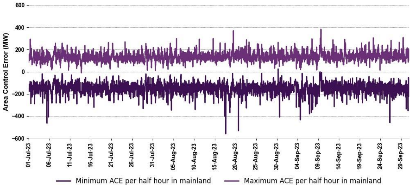
Figure 12 Minimum and maximum ACE per half-hour in mainland NEM
