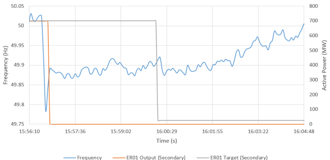
Figure 14 Frequency disturbance following Eraring Unit 1 generator trip
