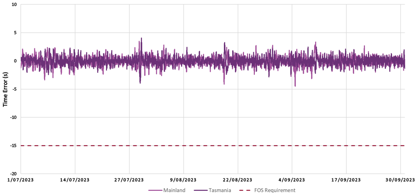
Figure 6 Time error in the mainland and Tasmania in Q3 2023
