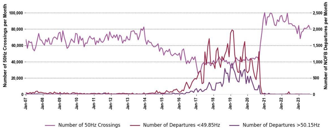
Figure 3 Monthly mainland frequency crossings
