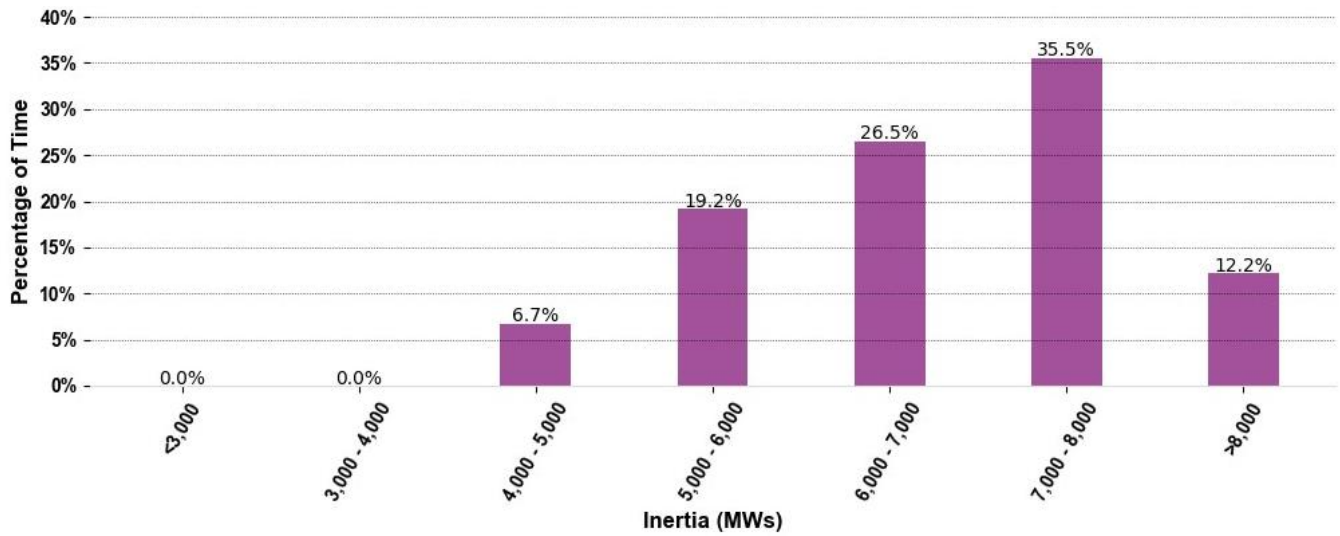
Figure 11 Distribution of Tasmania inertia in Q2 2023
