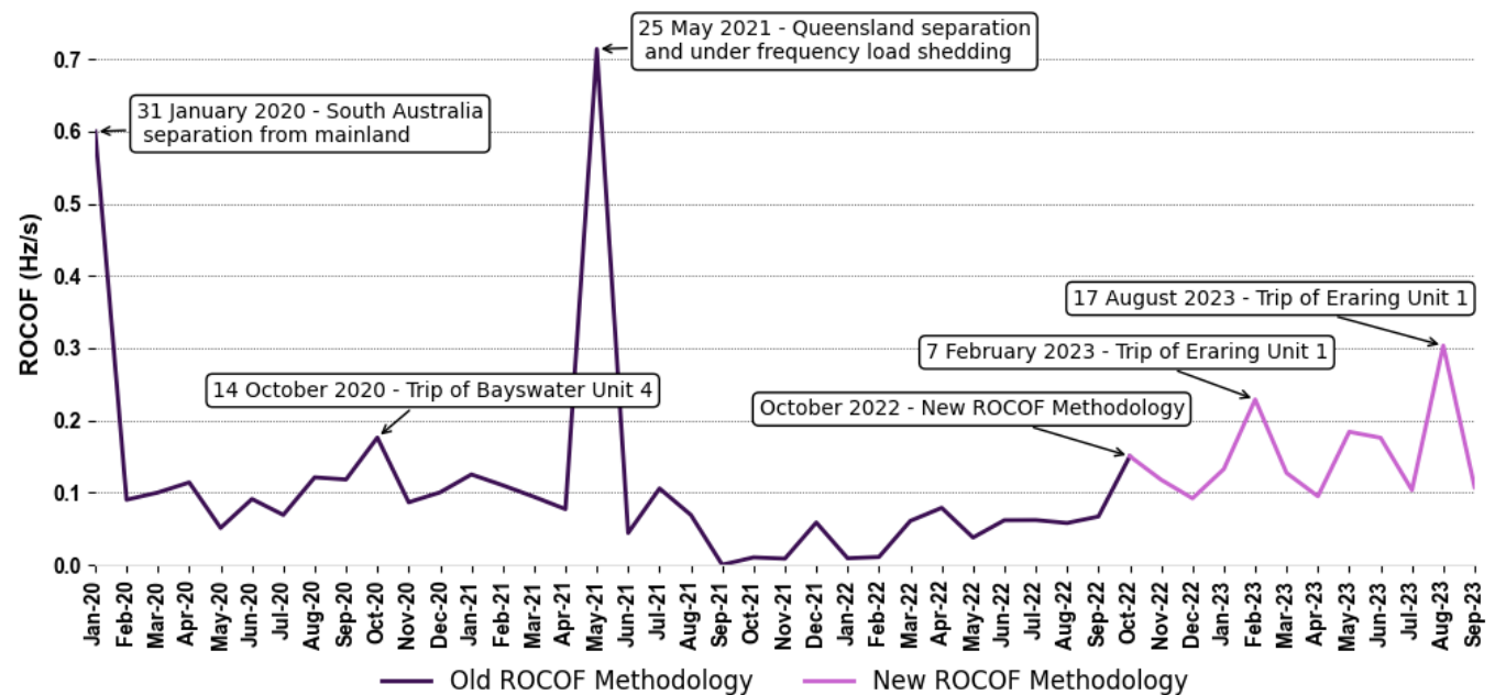
Figure 8 Monthly maximum RoCoF recorded in any mainland region in 2020-23
