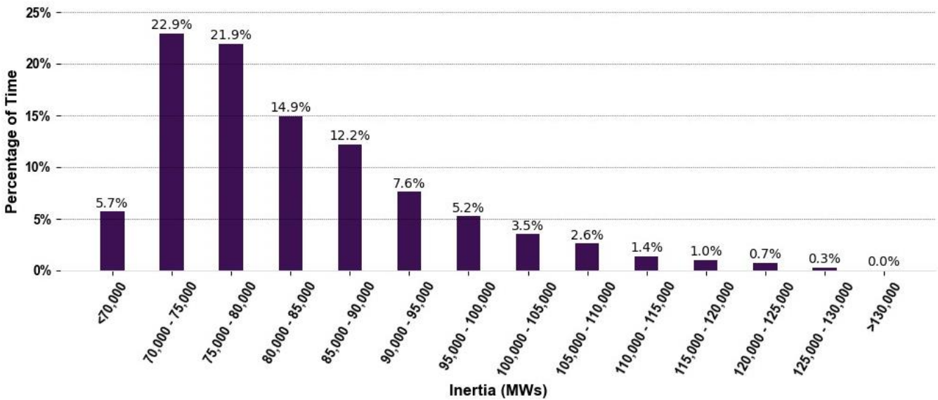
Figure 10 Distribution of mainland inertia in Q3 2023
