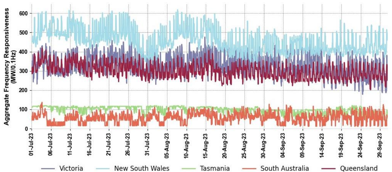
Figure 4 Estimated aggregate frequency responsiveness in NEM regions
