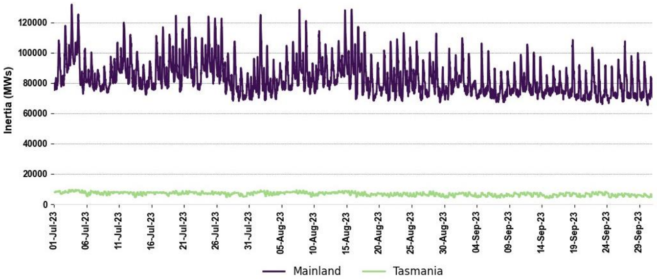
Figure 9 Time series mainland and Tasmania inertia in Q3 2023
