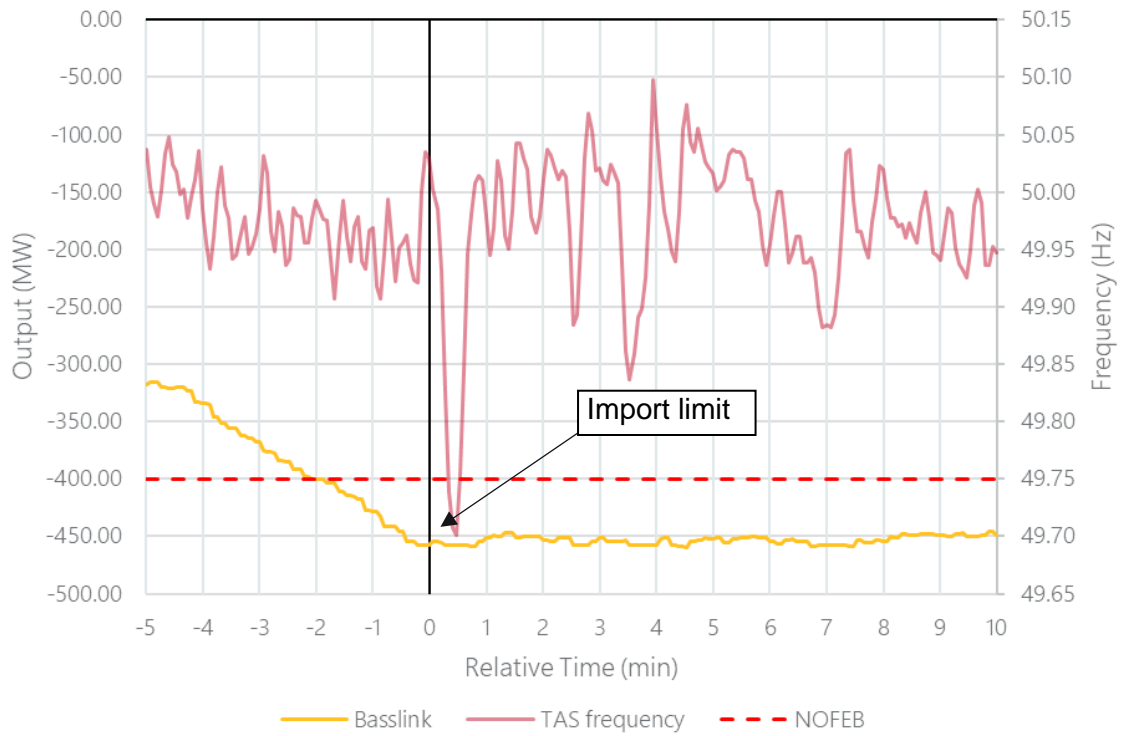
Figure 7 FOS exceedance in Tasmania on 29 September
