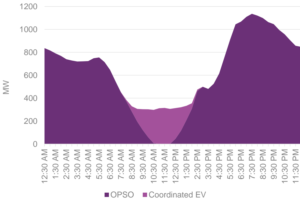
Figure 29 Adding coordinated EV charging
