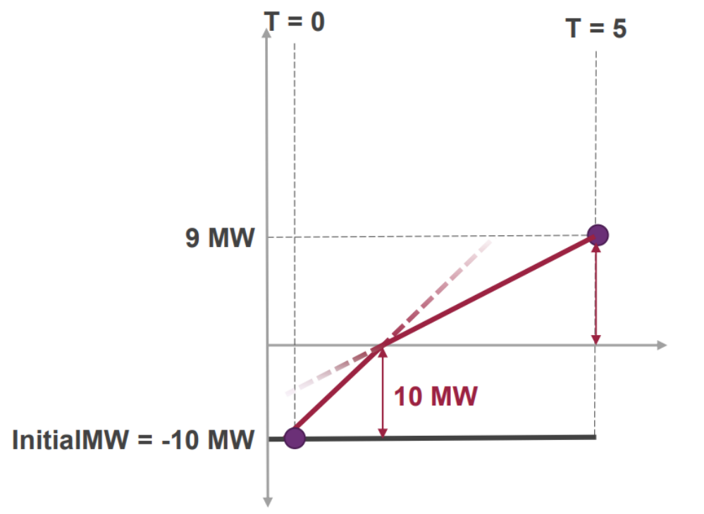
Figure 1: Composite ramp rate example
