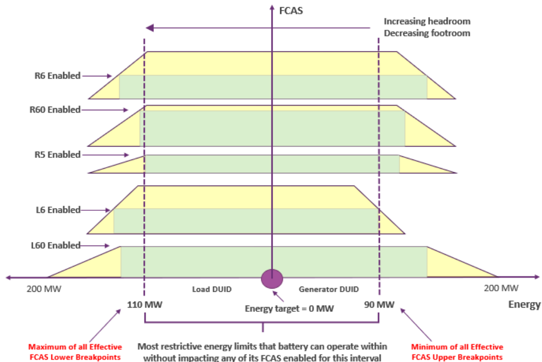
Figure 5 Operating Limits based on the most restrictive Contingency FCAS breakpoints
