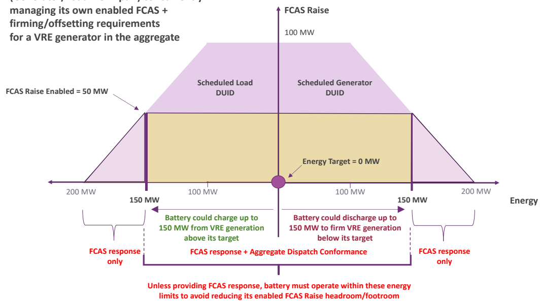
Figure 4 Operating Limits for managing Contingency FCAS and Aggregated Dispatch in a Mixed Aggregate
