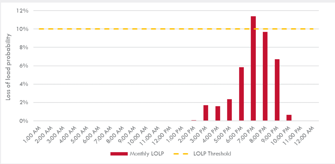
Figure 7 Time of day probability of lost load assessment (all identified months)
