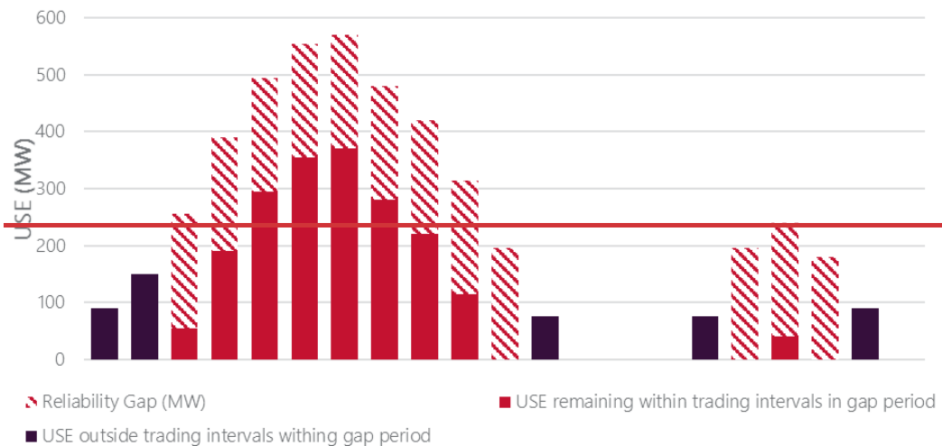
Figure 8 — Conceptual example of the forecast reliability gap
