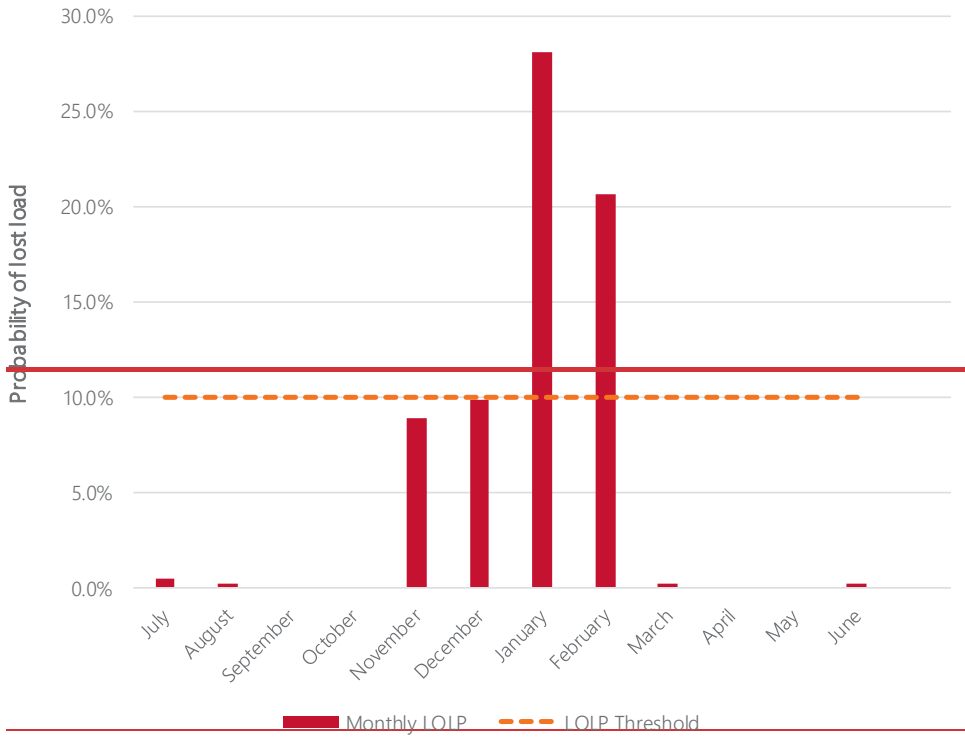
Figure 5 — Monthly probability of lost load assessment
