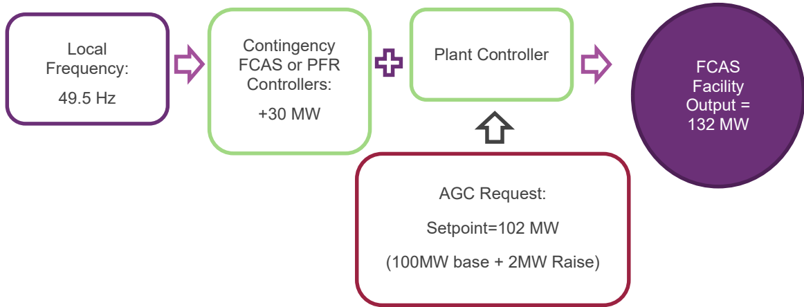
Figure 6 Figure 10 Co-ordinated output for Ancillary Service FCAS Facility at 100 MW given Raise Regulation FCAS request of 2 MW while responding with 30 MW to a Frequency Disturbance
