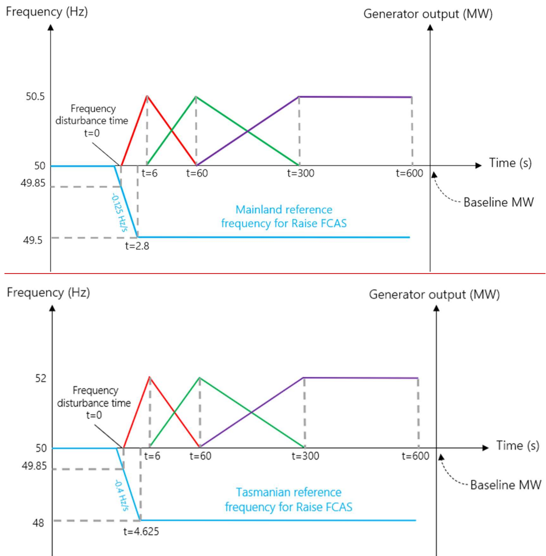
Figure 4 Figure 6 Measurement timeframes for Raise Contingency FCAS for the Mainland and Tasmania
