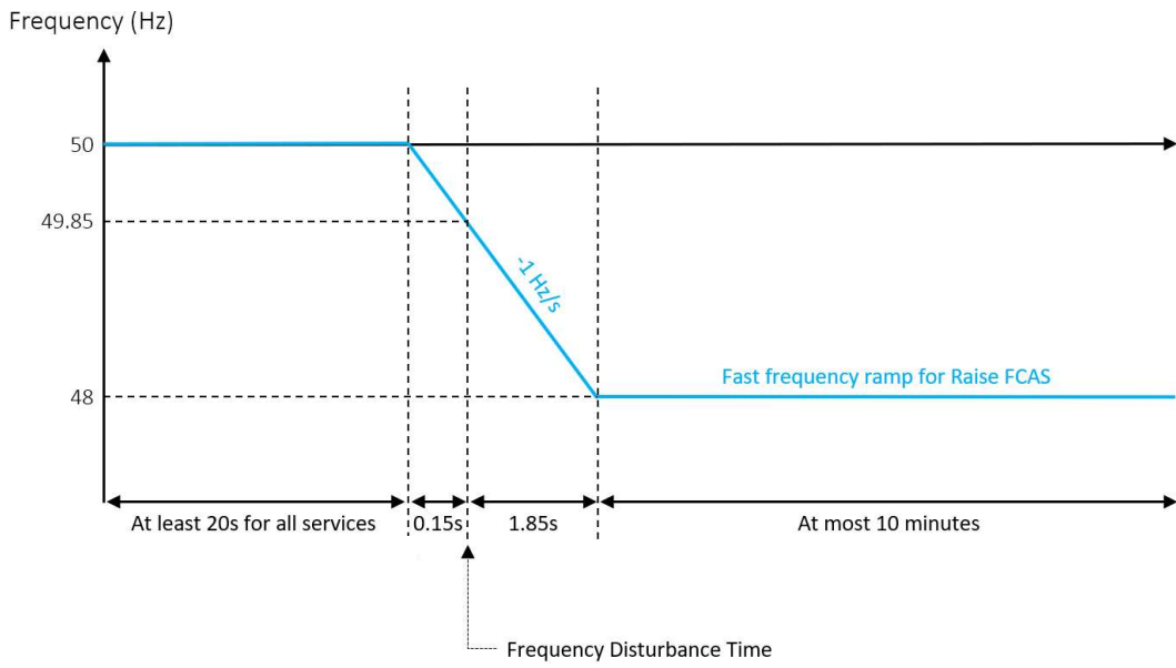
Figure 5 Fast Frequency Ramp for Tasmania
