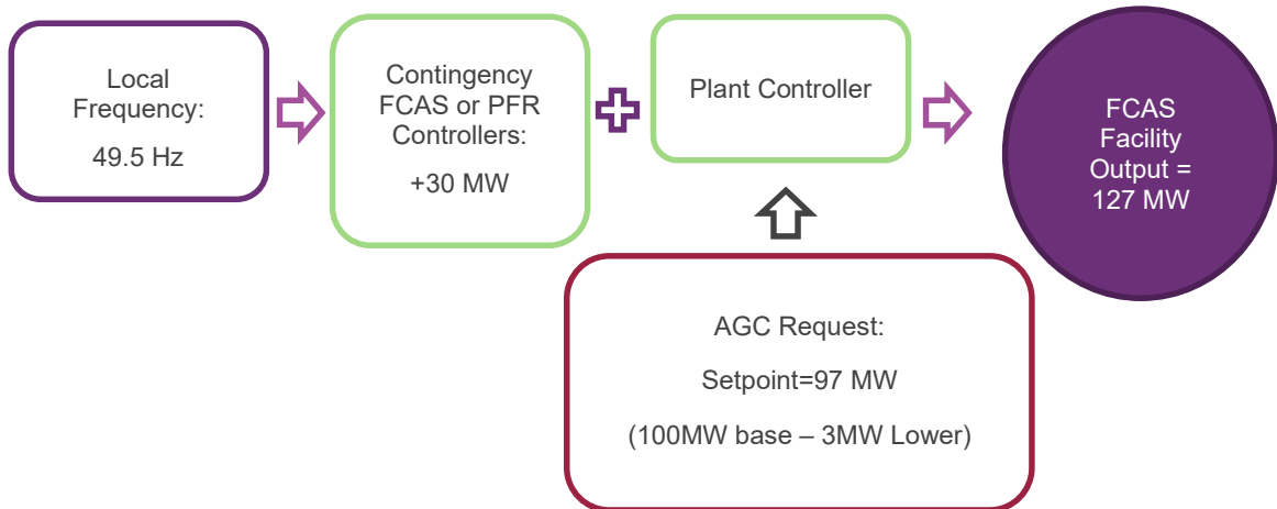
Figure 7 Figure 11 Co-ordinated output for Ancillary Service FCAS Facility at 100 MW given Lower Regulation FCAS request of 3 MW while responding with 30 MW to a Frequency Disturbance
