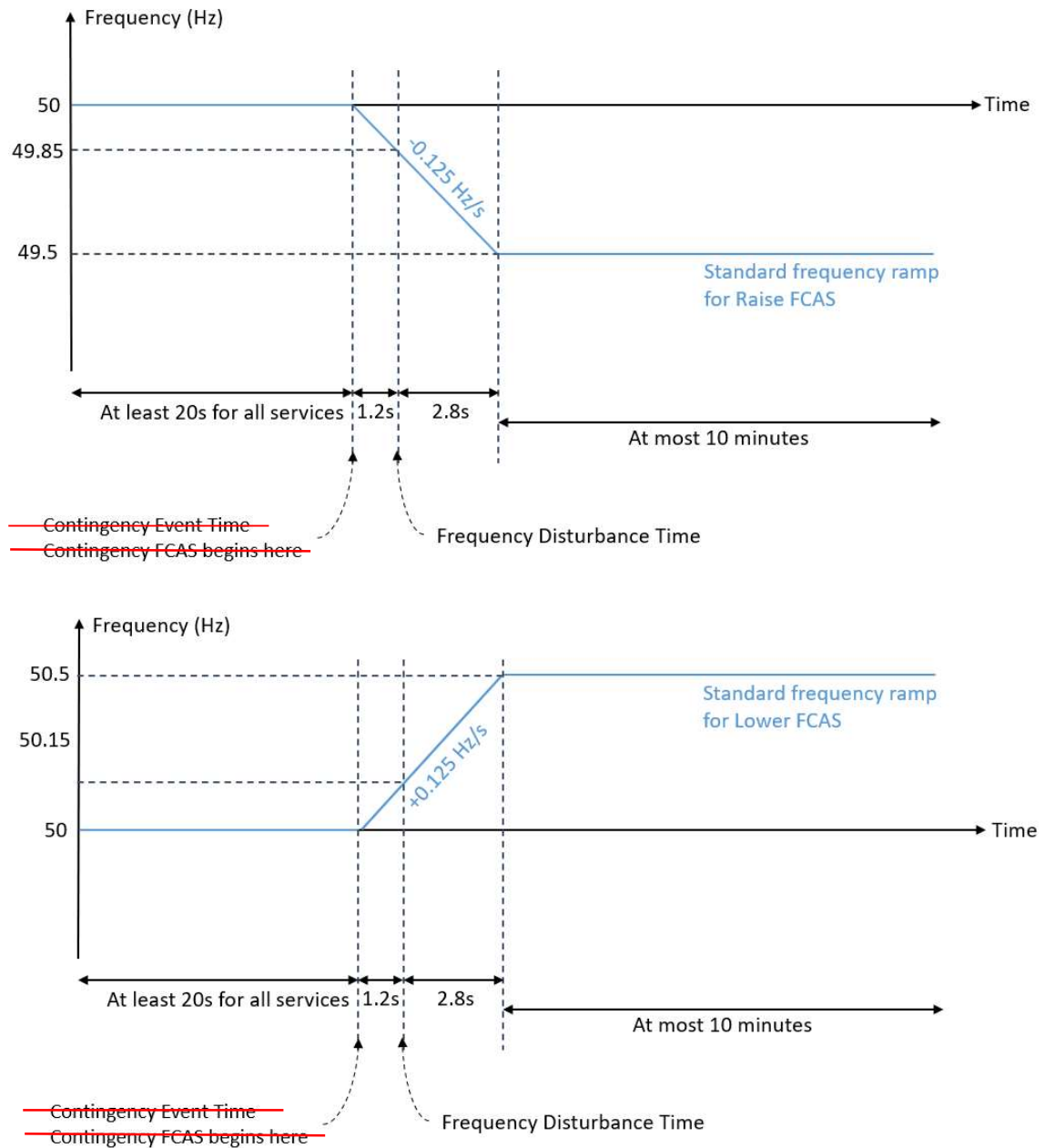
Figure 2 Standard Frequency Ramp for the Mainland
